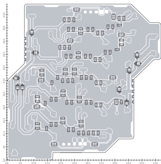
• BPF-A BOARD (BOTTOM VIEW)
