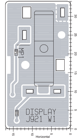
• KEY BOARD (BOTTOM VIEW)
