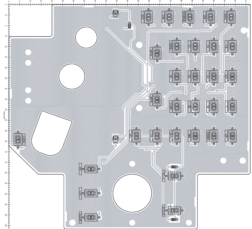
• TEN-KEY BOARD (TOP VIEW)
