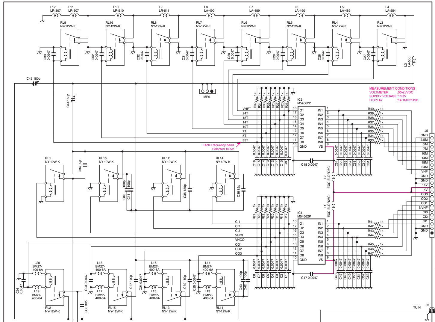
TUNER-A BOARD
