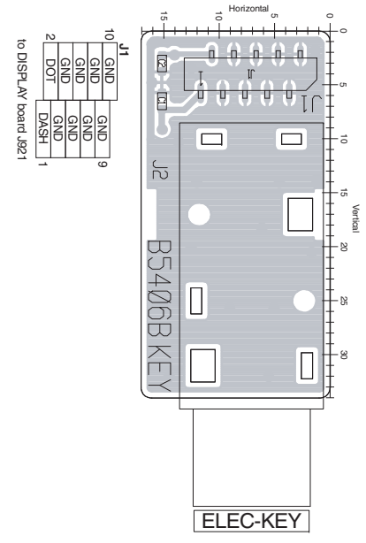
• KEY BOARD (TOP VIEW)
