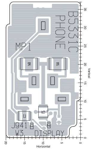
• PHONE BOARD (BOTTOM VIEW)
