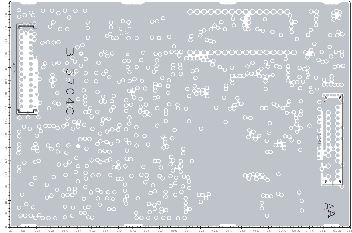
• DSP-A BOARD (BOTTOM VIEW)
