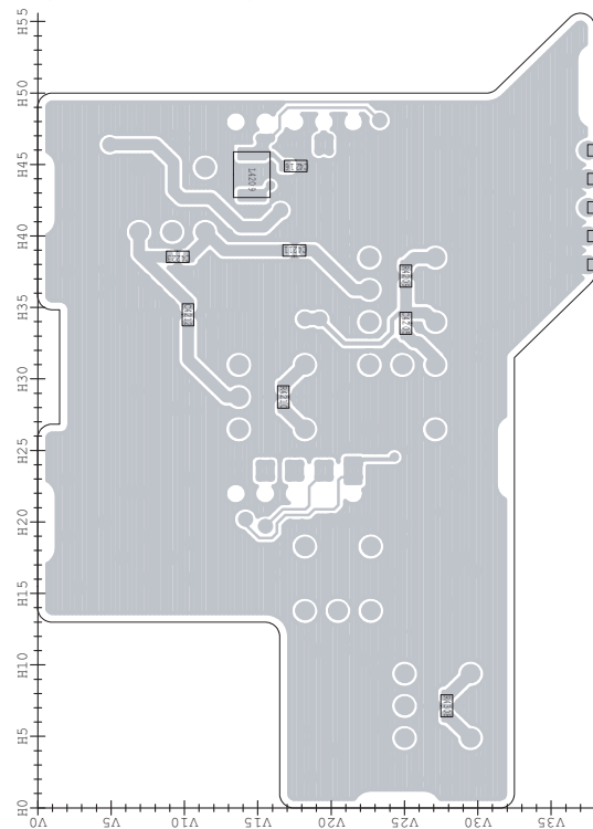
• PREAMP BOARD (BOTTOM VIEW)
