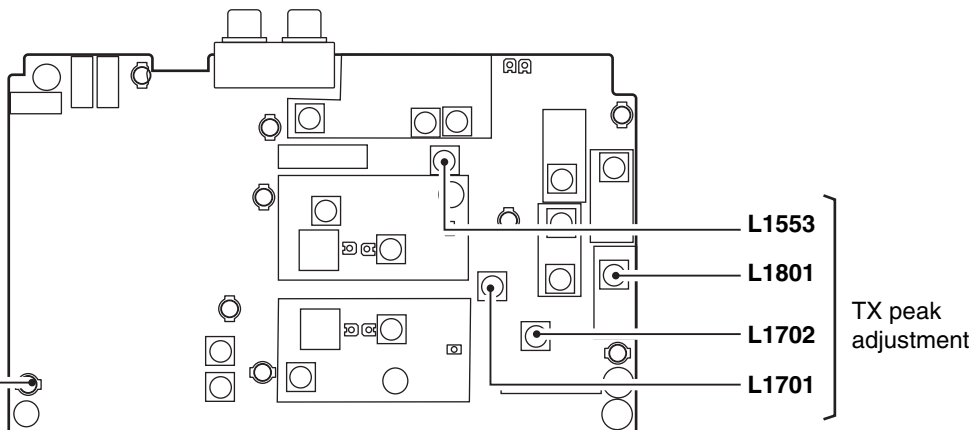
Bottom view of the transceiver
